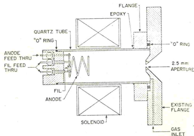
FIG. 1. Schematic drawing of the oscillating electron source.
